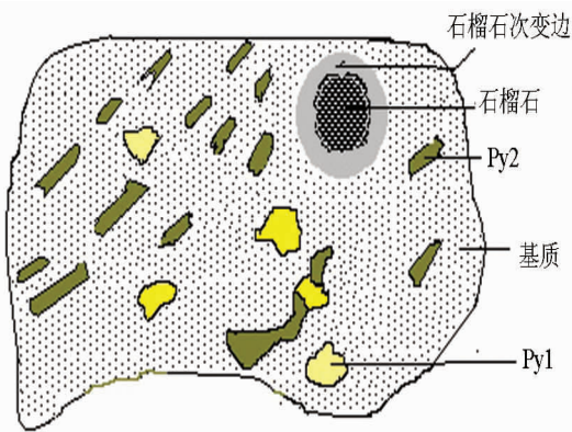
图 1 蒙阴橄榄岩捕虏体(9137)手标本素描(长 10cm) Fig.1 Sketch of peridotite xenolith hand specimen (Sp 9137) from Mengyin (specimen length=10cm)
